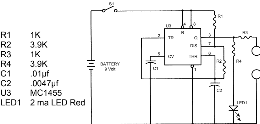
Fig. 93 Zapper schematic.
